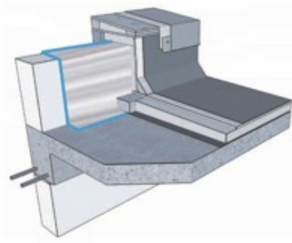
Roof-To-Wall Transition
