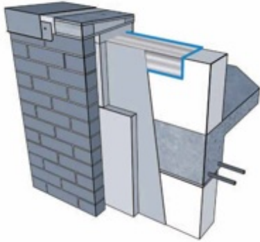
Parapet Transition Membrane
