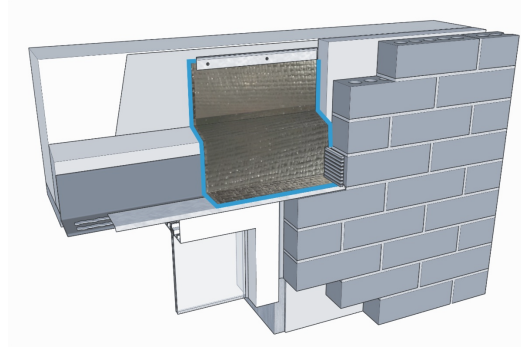
Window Head
