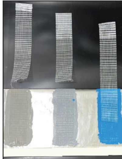
Test strips break while pulled off of the stainless steel membrane due to superior adhesion, >15 psi
