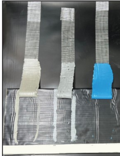
Test strips are easily pulled off of the peel & stick membrane with little resistance, <2 psi
