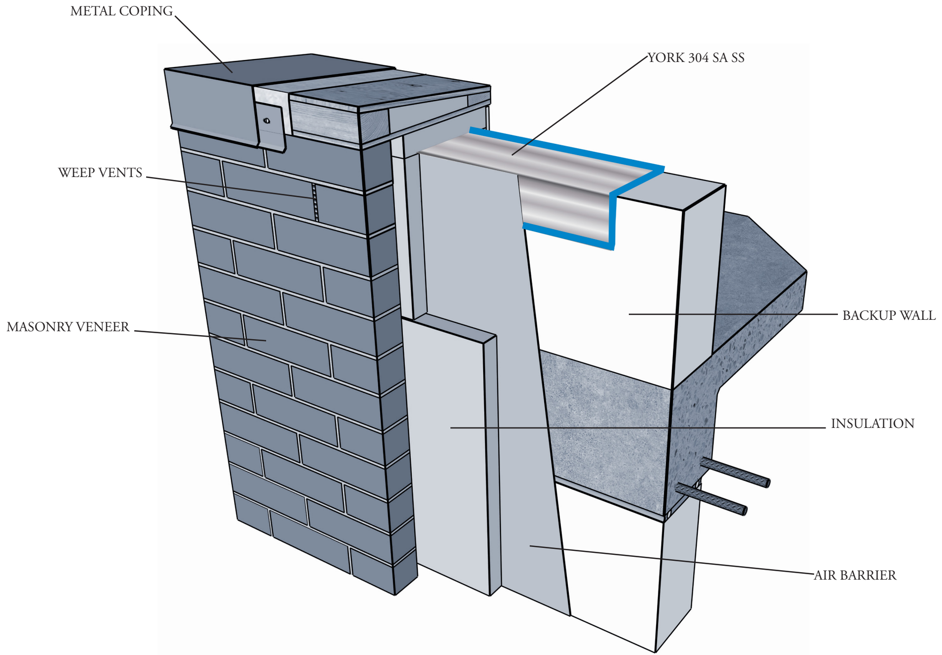
ROOF TO WALL PARAPET DETAIL YORK 304 SELF-ADHERING STAINLESS STEEL
