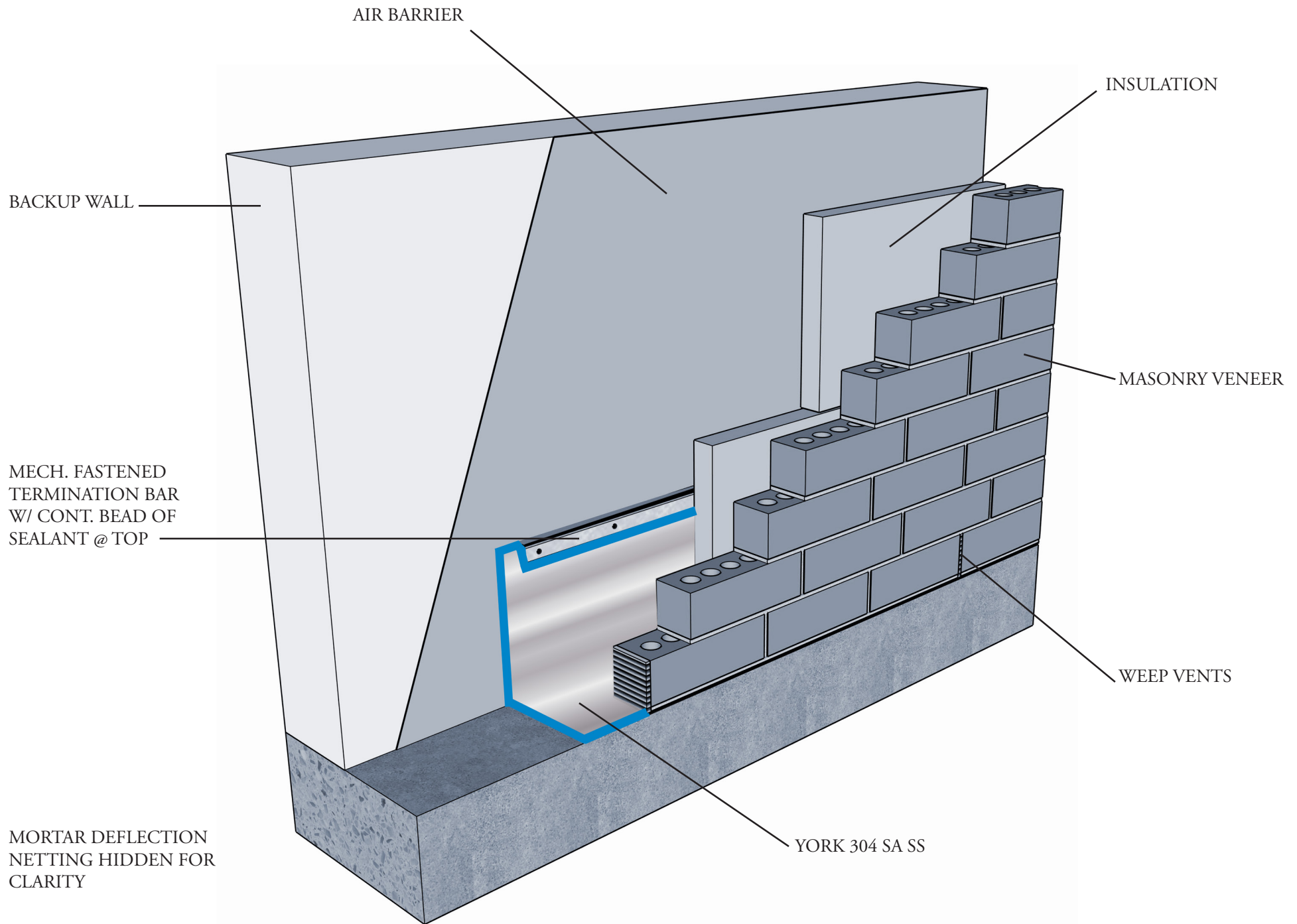
BASE OF WALL DETAIL YORK 304 SELF-ADHERING STAINLESS STEEL
