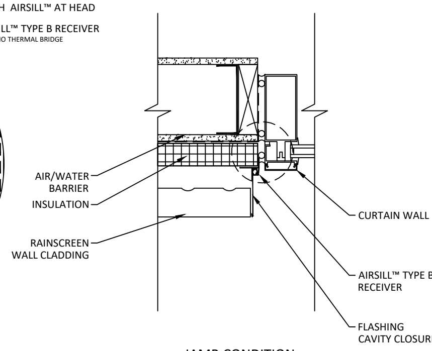
JAMB CONDITION
