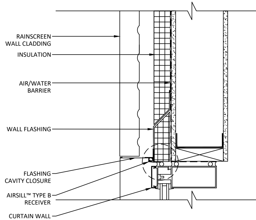
HEAD CONDITION
