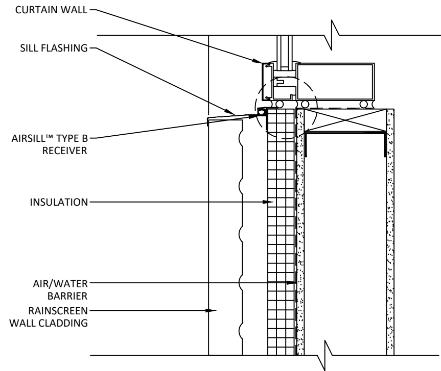
SILL CONDITION
